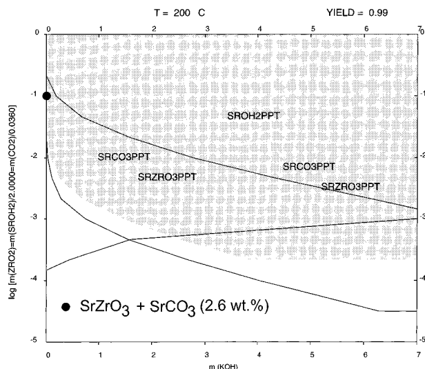
Figure 14. Calculated phase stability and yield diagram at 473 K for Sr/Zr = 2.0 using \text{Sr}(\text{OH})_2 as a source of Sr when the amount of \text{CO}_2 in the starting materials (i.e., hydrous \text{ZrO}_2 ) is equal to 0.036 times the amount of \text{ZrO}_2 . The solid circle denotes experimental conditions for which \text{SrZrO}_3 contaminated with 2.6 wt % of \text{SrCO}_3 was obtained.
