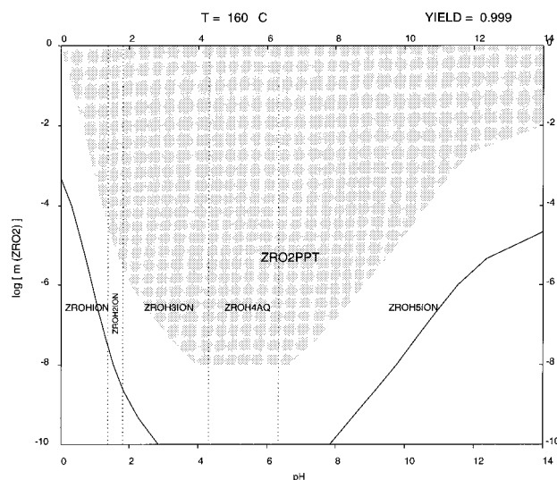
Figure 2. Calculated phase stability diagram for the Zr hydrothermal system at 433 K. The symbols ZRO2PPT, ZROH2ION, ZROH3ION, ZROH4AQ, and ZROH5ION denote \text{ZrO}_2(\text{s}) , \text{ZrOH}^{3+} , \text{Zr}(\text{OH})_2^{2+} , \text{Zr}(\text{OH})_3^+ , \text{Zr}(\text{OH})_4(\text{aq}) , and \text{Zr}(\text{OH})_5^- , respectively.
