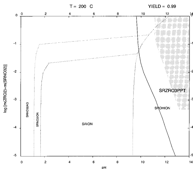
Figure 4. Calculated phase stability and yield diagram for the Sr–Zr hydrothermal system at 473 K for Sr/Zr = 1.0 using \text{Sr}(\text{NO}_3)_2 as a source of strontium.
