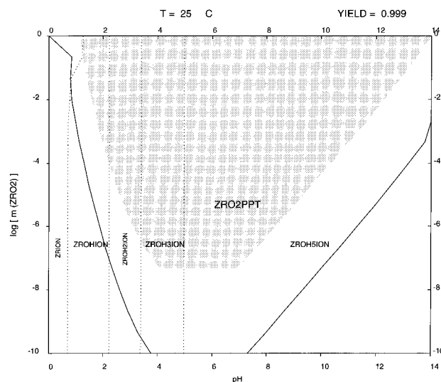
Figure 1. Calculated phase stability and yield diagram for the Zr hydrothermal system at 298 K. The symbols ZRO2PPT, ZRION, ZROH2ION, ZROH3ION, and ZROH5ION denote \text{ZrO}_2(\text{s}) , \text{Zr}^{4+} , \text{ZrOH}^{3+} , \text{Zr}(\text{OH})_2^{2+} , \text{Zr}(\text{OH})_3^+ , and \text{Zr}(\text{OH})_5^- , respectively.
