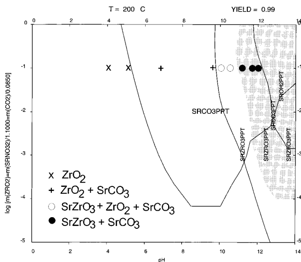
Figure 12. Calculated phase stability and yield diagram at 473 K for Sr/Zr = 1.1 using Sr(NO 3 ) 2 as a source of strontium when the amount of CO 2 in the starting materials is equal to 0.085 times the amount of ZrO 2 . The symbols denote experimental conditions for which the following products were obtained: (x) ZrO 2 , (+) SrCO 3 + ZrO 2 , (o) SrZrO 3 + ZrO 2 + SrCO 3 , (●) SrZrO 3 + SrCO 3 .
