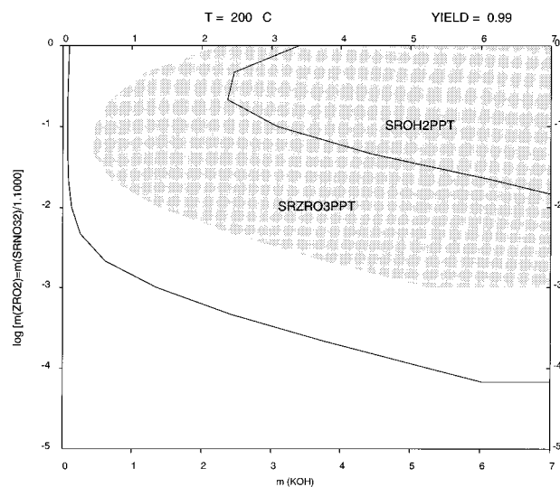
Figure 9. Calculated phase stability and yield diagram as a function of the input amount of KOH at 473 K for Sr/Zr = 1.1 using \text{Sr}(\text{NO}_3)_2 as a source of strontium.
