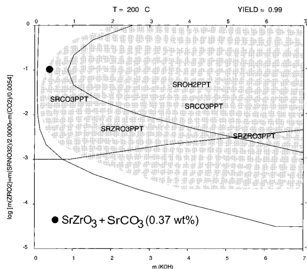
Figure 13. Calculated phase stability and yield diagram at 473 K for Sr/Zr = 2.0 using Sr(NO 3 ) 2 as a source of strontium when the amount of CO 2 in the starting materials (i.e., KOH) is equal to 0.0054 times the amount of ZrO 2 . The solid circle denotes experimental conditions for which SrZrO 3 contaminated with 0.37 wt % of SrCO 3 was obtained.
