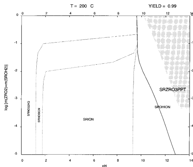
Figure 5. Calculated phase stability and yield diagram for the Sr–Zr hydrothermal system at 473 K for Sr/Zr = 1 using \text{Sr}(\text{OH})_2 as a source of strontium.
