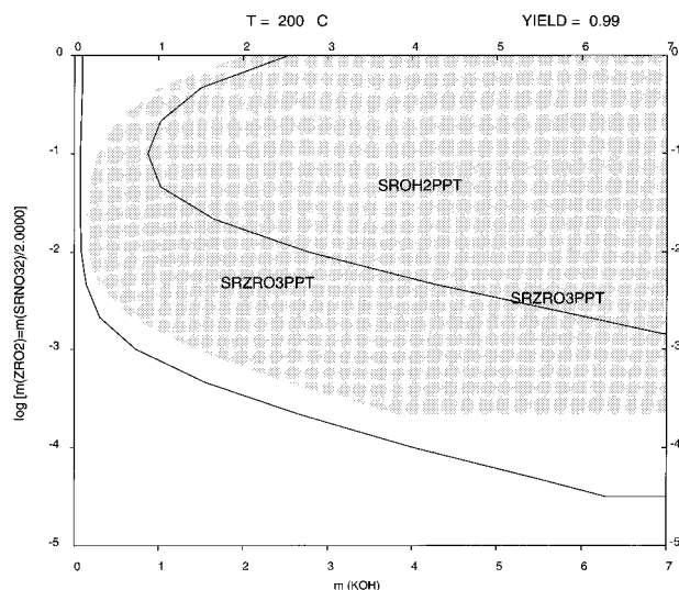
Figure 10. Calculated phase stability and yield diagram as a function of the input amount of KOH at 473 K for Sr/Zr = 2.0 using \text{Sr}(\text{NO}_3)_2 as a source of strontium.
