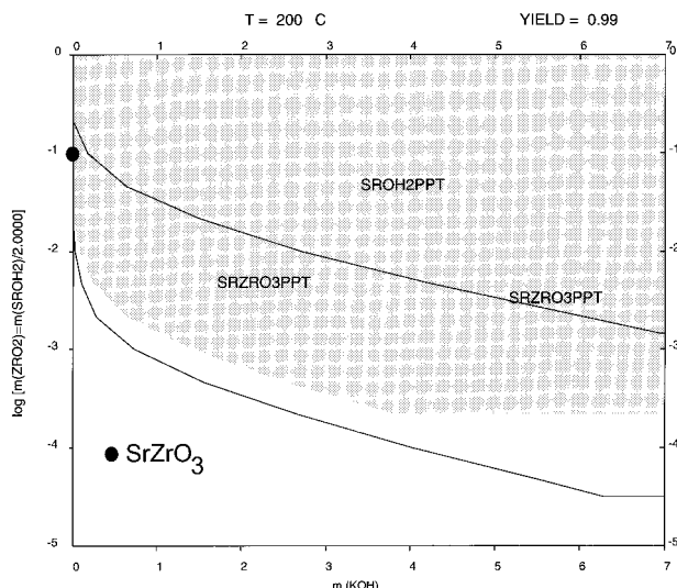
Figure 11. Calculated phase stability and yield diagram as a function of the input amount of KOH at 473 K for Sr/Zr = 2.0 using Sr(OH) 2 as a source of strontium. The solid circle denotes experimental conditions for which phase-pure SrZrO 3 was obtained.
