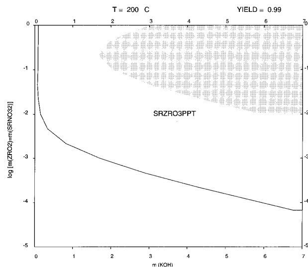
Figure 6. Calculated phase stability and yield diagram as a function of the input amount of KOH at 473 K for Sr/Zr = 1 using \text{Sr}(\text{NO}_3)_2 as a source of strontium.
