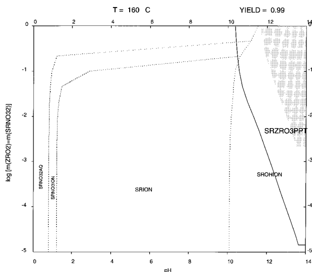
Figure 3. Calculated phase stability and yield diagram for the Sr–Zr hydrothermal system at 433 K for Sr/Zr = 1.0 using \text{Sr}(\text{NO}_3)_2 as a source of strontium. The symbols \text{SrNO}_3\text{2AQ} , \text{SrNO}_3\text{ION} , \text{SRION} , \text{SROHION} , and \text{SRZRO}_3\text{PPT} denote \text{Sr}(\text{NO}_3)_2(\text{aq}) , \text{SrNO}_3^{3+} , \text{Sr}^{2+} , and \text{SrOH}^+ , respectively.
